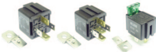
4 Blade relay 5 Blade relay 4 Blade fused relay
